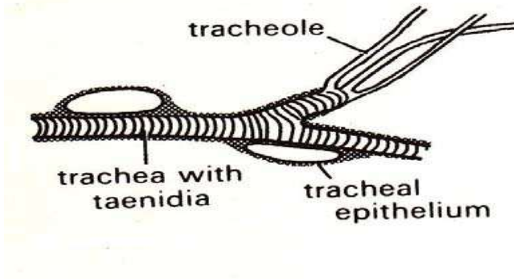
Structure of trachea
