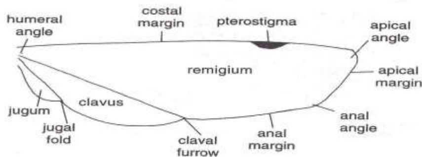
Fig. Insect wing areas
